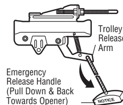
LOCKOUT POSITION
