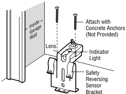
Figure 4 FLOOR MOUNT (RIGHT SIDE)
