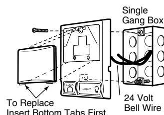
Figure 2 PRE-WIRED INSTALLATION
