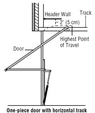
One-piece door with horizontal track
