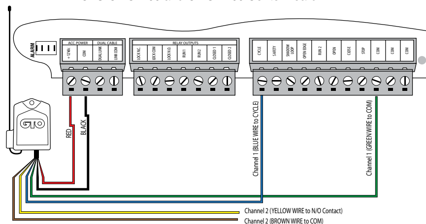
GTO GP-SL100 and GP-SW100 Contol Board
