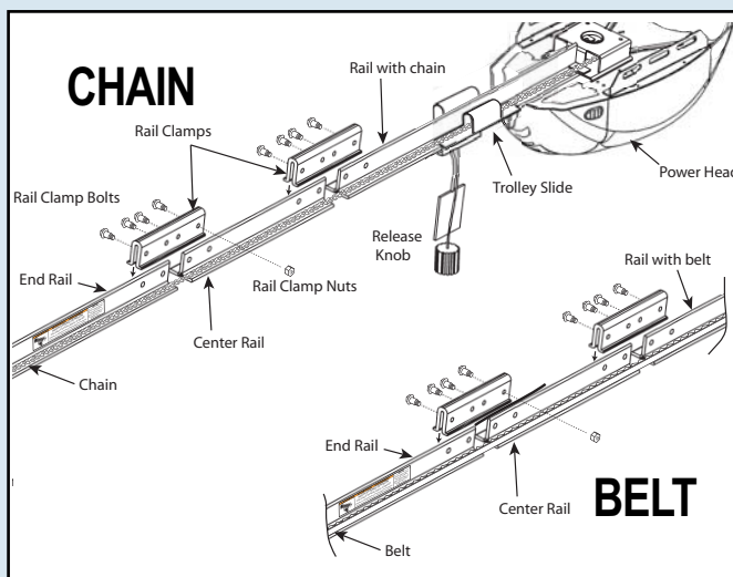
FIG. 1-3 Split Rail assembly.
