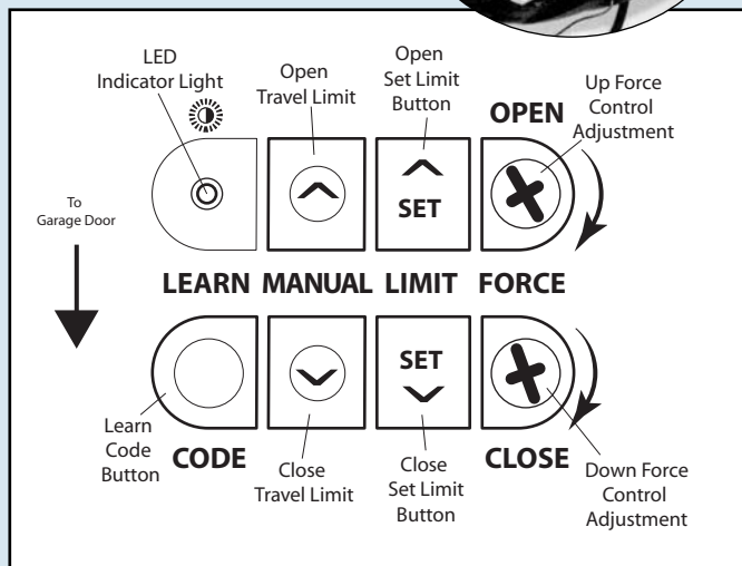
FIG. 6-1 Limit controls.
