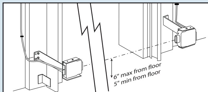
FIG. 5-4 Check Safe-T-Beam® alignment.
