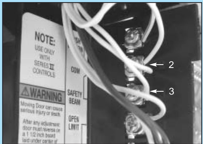
FIG. 3-8 Terminal attachments at power head.
