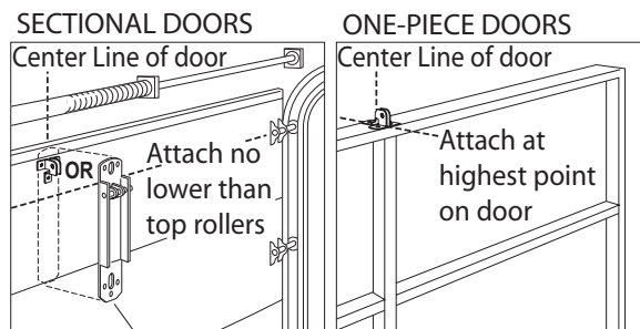
Figure 19 Attach Door Bracket
