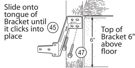
Figure 25 Install Safe-T-Beams®
