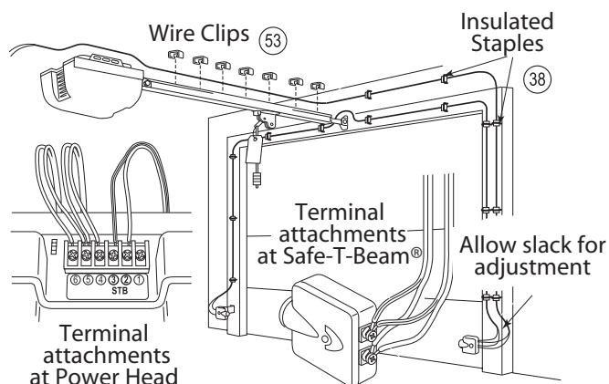
Figure 29 Wiring Method B
