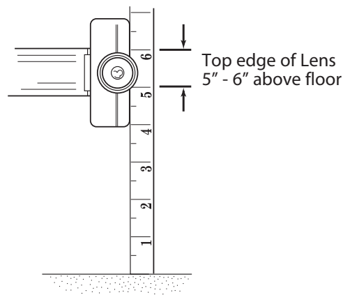
Figure 26 Final Check Safe-T-Beams®
