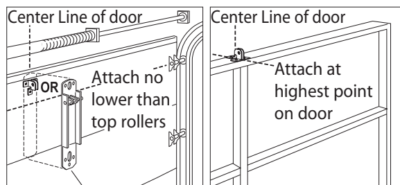
Optional Door Operator Bracket (not included)
