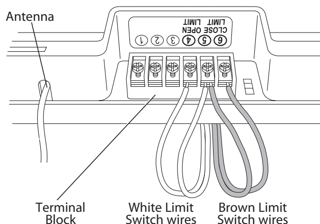
Figure 15 Connect Limit Switch Wires to Power Head Terminal Block
