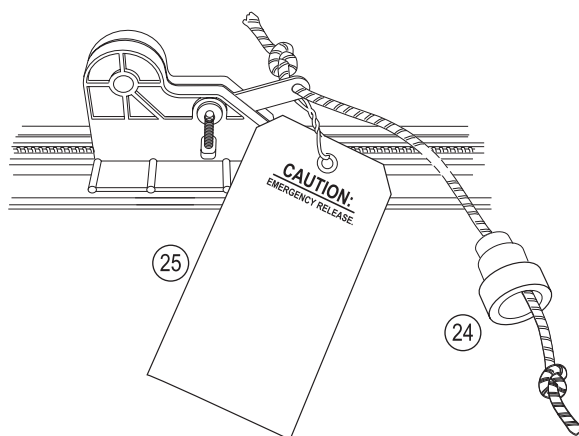
Figure 16 Attach Emergency Release Cord and Knob
