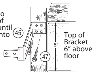
Figure 24 Install Safe-T-Beams®
