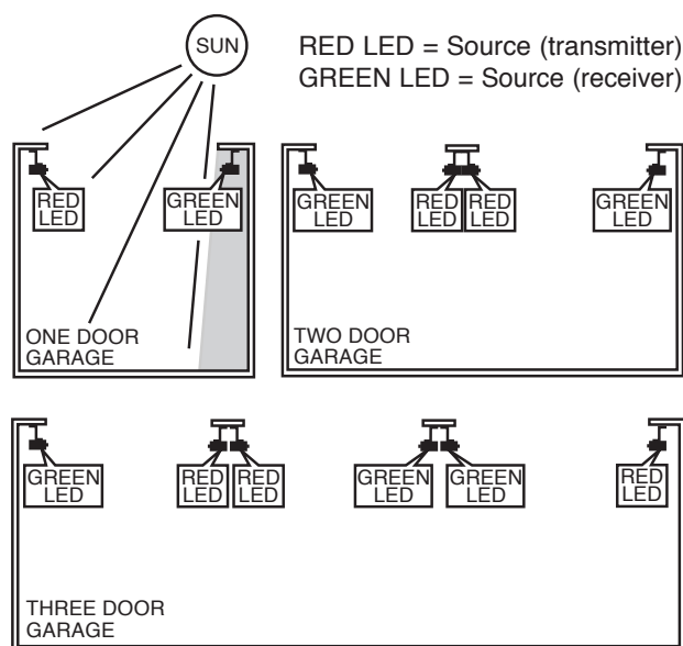
Figure 25 Source/sensor Locations
