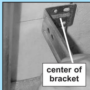
FIG. 4-2 Mounting brackets.
