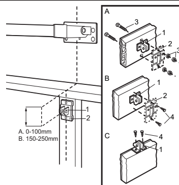
C. One-piece door optional Fasten with wood screws (4).
