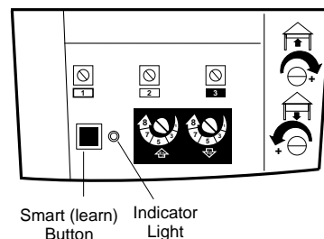
Figure 2 SECURITY+ Garage Door Opener
