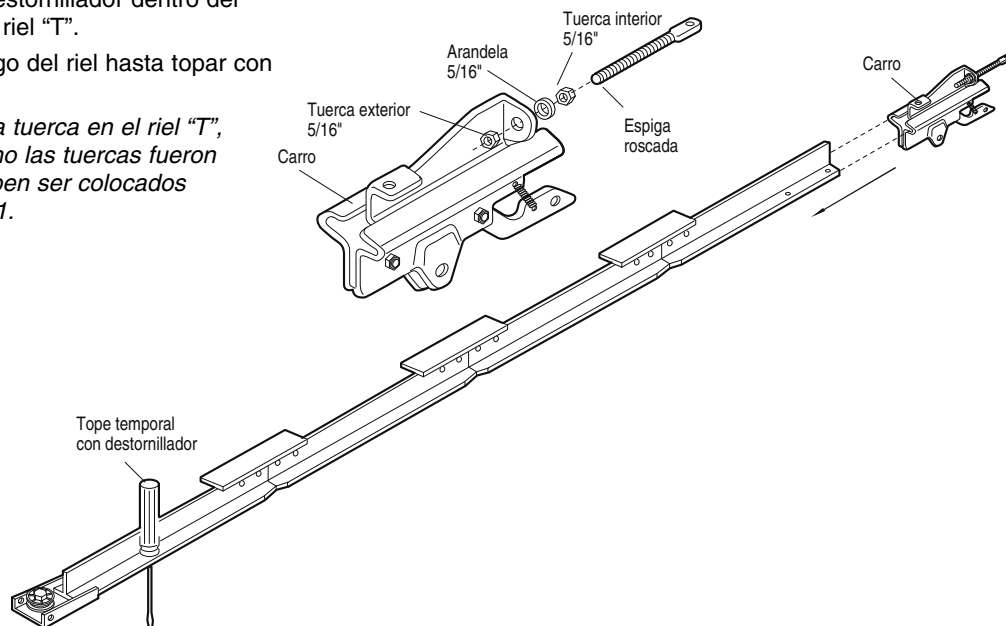
Arandela 5/16"
