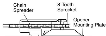
Sectional Doors 8-Tooth Sprocket Application (6-tooth sprocket can be used if slower travel speed is desired.)
