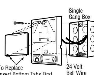
Figure 2 PRE-WIRED INSTALLATION
