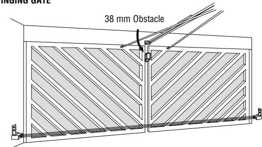
SWINGING GATE
