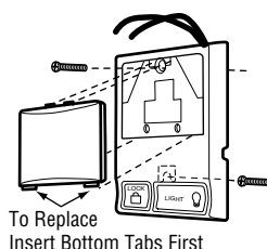
Figure 1 STANDARD INSTALLATION
