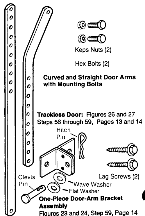
Sectional Door-Arm Bracket and Mounting Screws. Figure 14, Page 10, Steps 31 and 32
