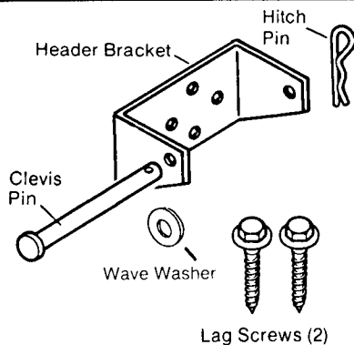
Header Bracket Assembly See Figures 8 and 23 Steps 16 and 59 Pages 8 and 14
