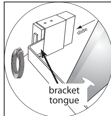
FIG. 4-3 Attach sensors to brackets
