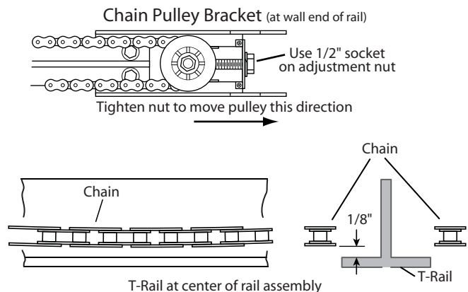
FIG. 1-3 Chain adjustment.
