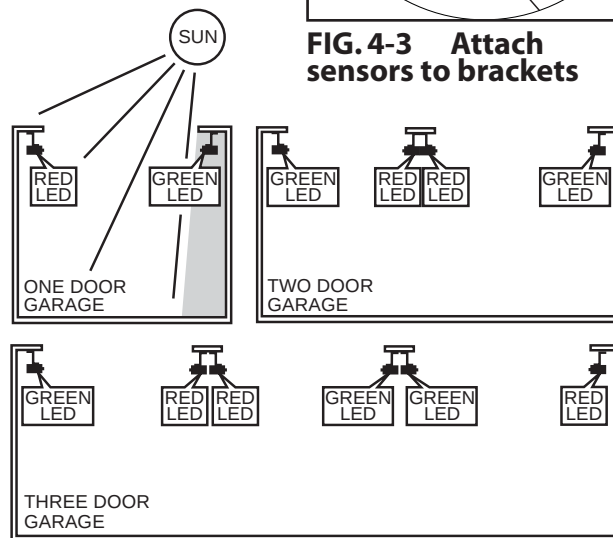
FIG. 4-4 Safe-T-Beam® source and sensor locations
