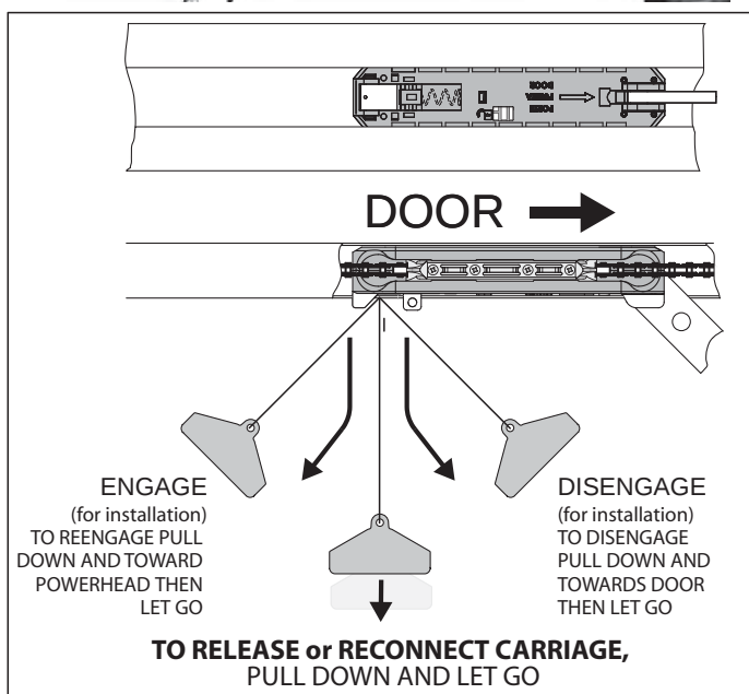
FIG. 6-4 Carriage (cut away view)
