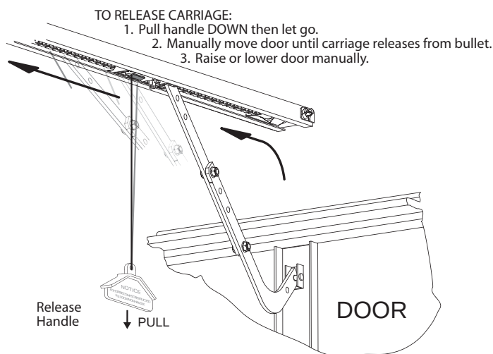
FIG. 6-3 Carriage Release
