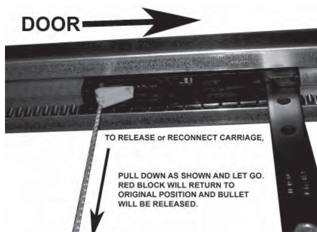
FIG. 6-3 Carriage Release
