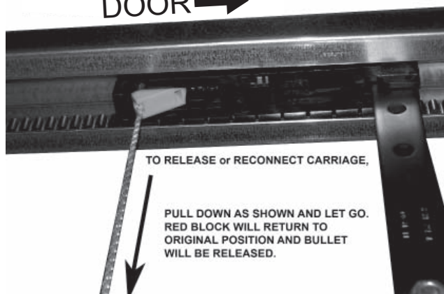
FIG. 6-3 Carriage Release
