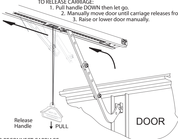
FIG. 6-3 Carriage Release
