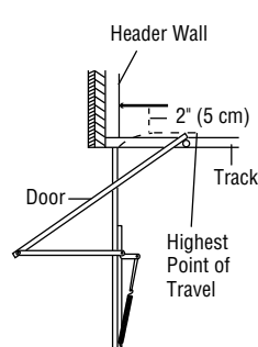
One-piece door with horizontal track
