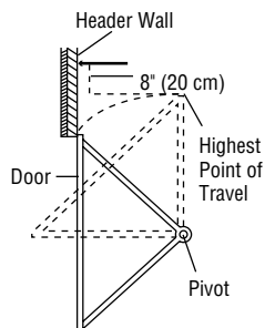
One-piece door without track: pivot hardware
