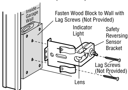
Figure 3 WALL MOUNT (RIGHT SIDE)
