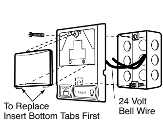
Figure 2 PRE-WIRED INSTALLATION
