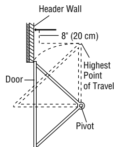
One-piece door without track: pivot hardware
