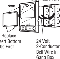
Figure 4 REMOVE COVER
