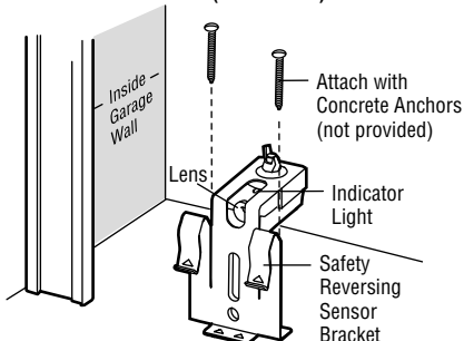
Figure 4 FLOOR MOUNT (RIGHT SIDE)
