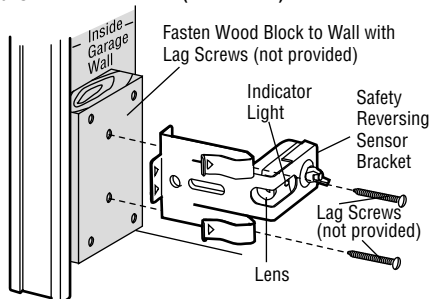
Figure 2 WALL MOUNT (RIGHT SIDE)
