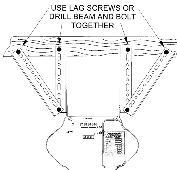
BEAM MOUNT
