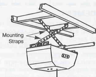
GARAGE WITH OPEN BEAMS
