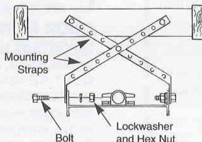
GARAGE WITH OPEN BEAMS
