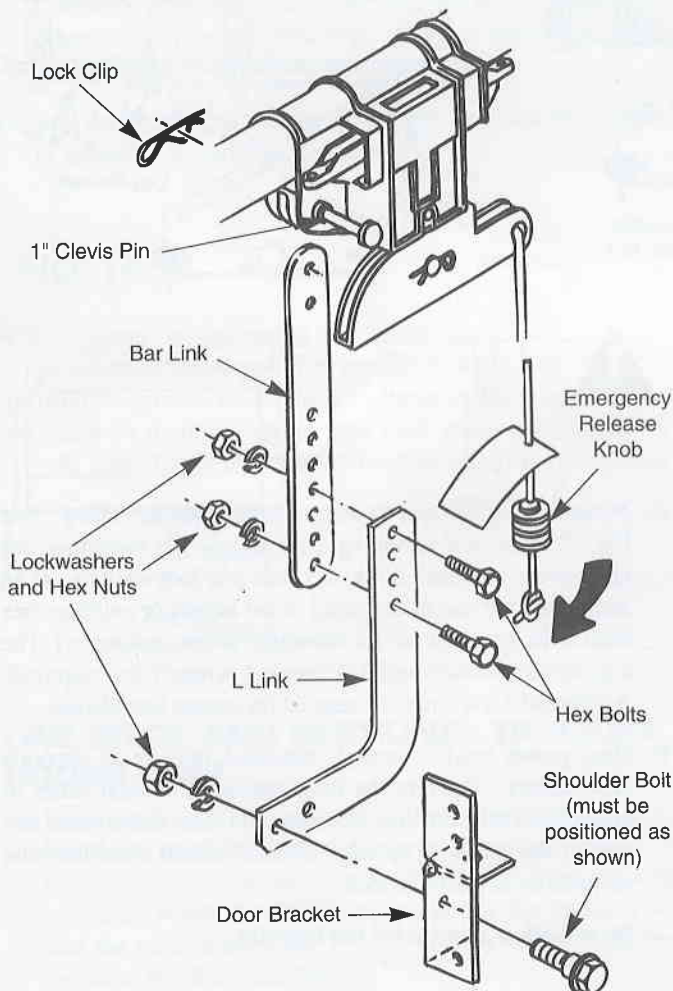
FIG. 21 TRACKED-TYPE DOOR MOUNTING
